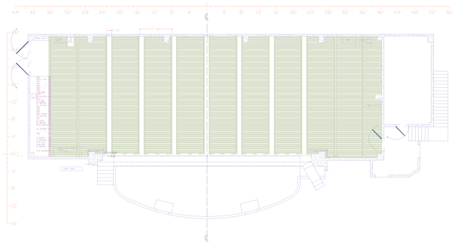
THE FOX THEATER OF BAKERSFIELD, CA Ground Plan of Stage with Grid Scale: 1/4"=1'-0" | 12-2-66 | Dr. R. Finnell
